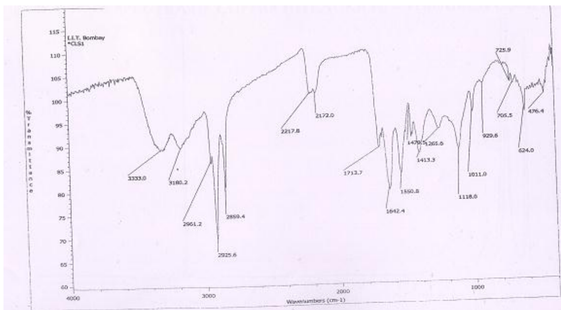
Fig. (3). IR Spectra of complex ( \text{CL}_{\text{rt}}\text{T} ).
