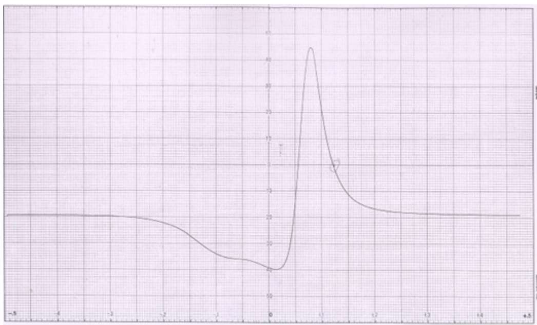
Fig. (5). ESR Spectra of complex (CL π T).
