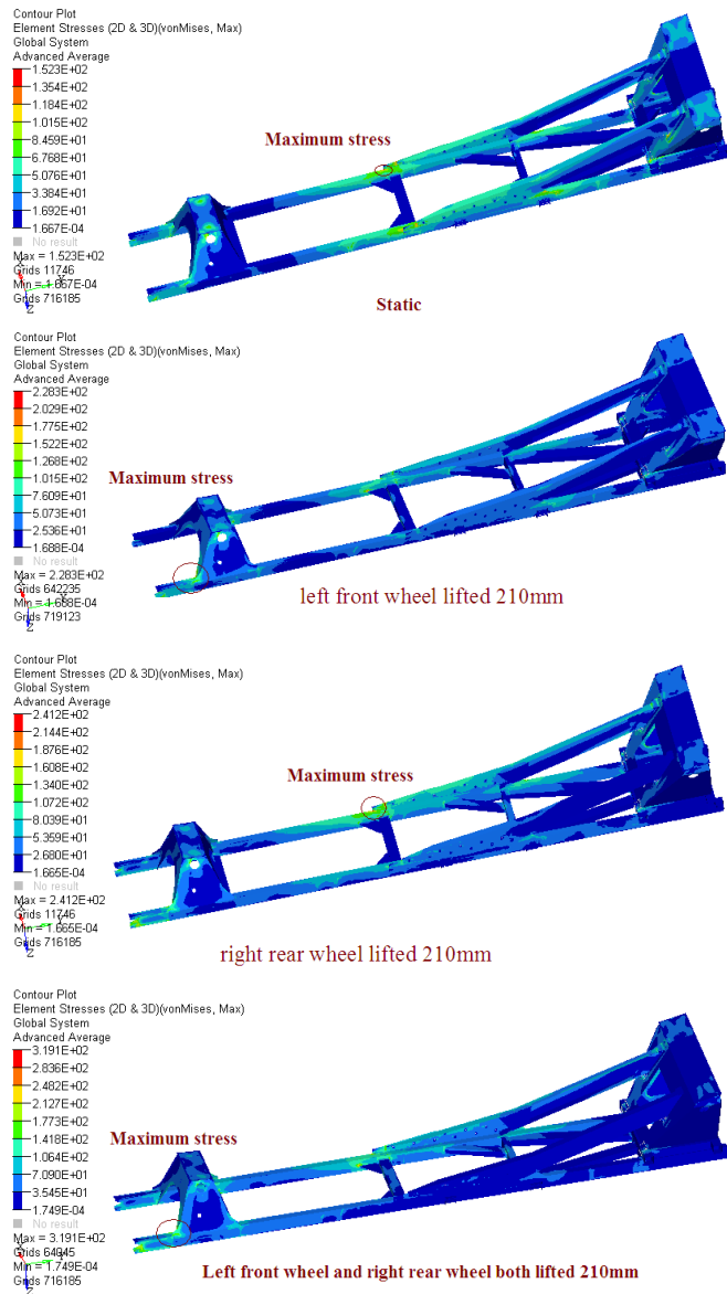
Fig. (2). Shows a auxiliary frame stress nephogram under full load condition.
