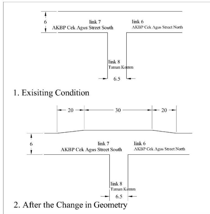
Fig. (3). Geometric improvement at Taman Kenten intersection.
